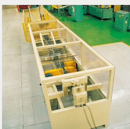
靜水壓重複彎曲試驗 Flexural Test for Hydrostatic Pressure
