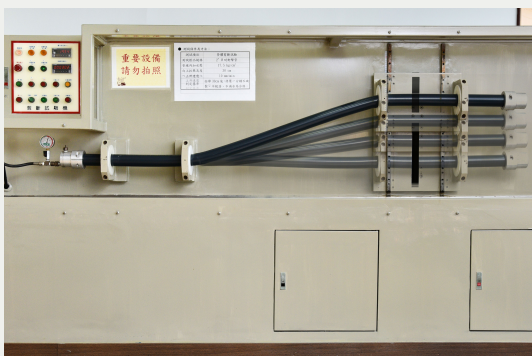
管體剪斷試驗 Cutting Test for PVC-U Pipe
