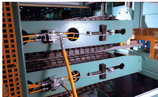
引取機 Haul-off equipment
